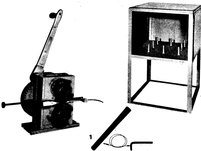
type II bench model manual swaging tool kit — part no. M2-K*
